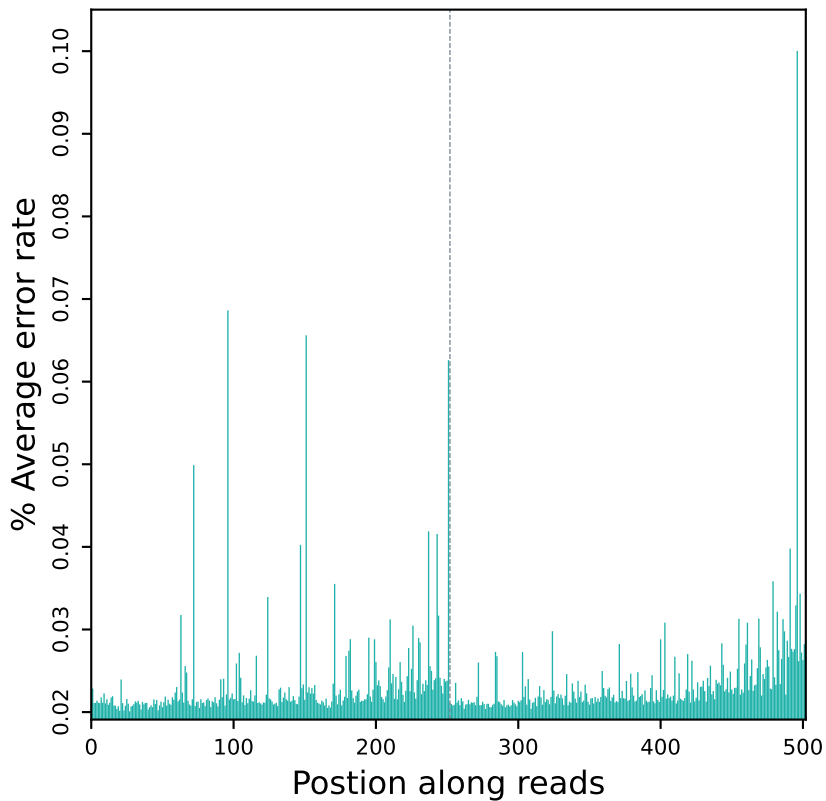
Error rate distribution along reads (R10110)
